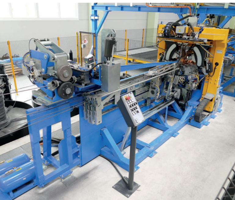
With the highly flexible VGA Versa lattice girder welding machine, the lattice girders are produced "just in time", which enables Eder to achieve high savings potential in logistics, storage costs and waste.
